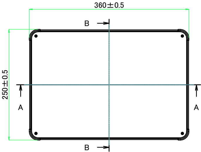
E view
